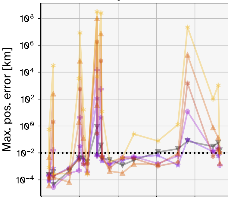
Integrator: RK10
