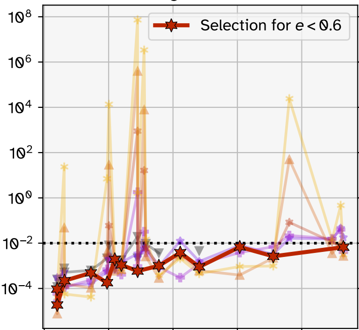
Integrator: RK12
