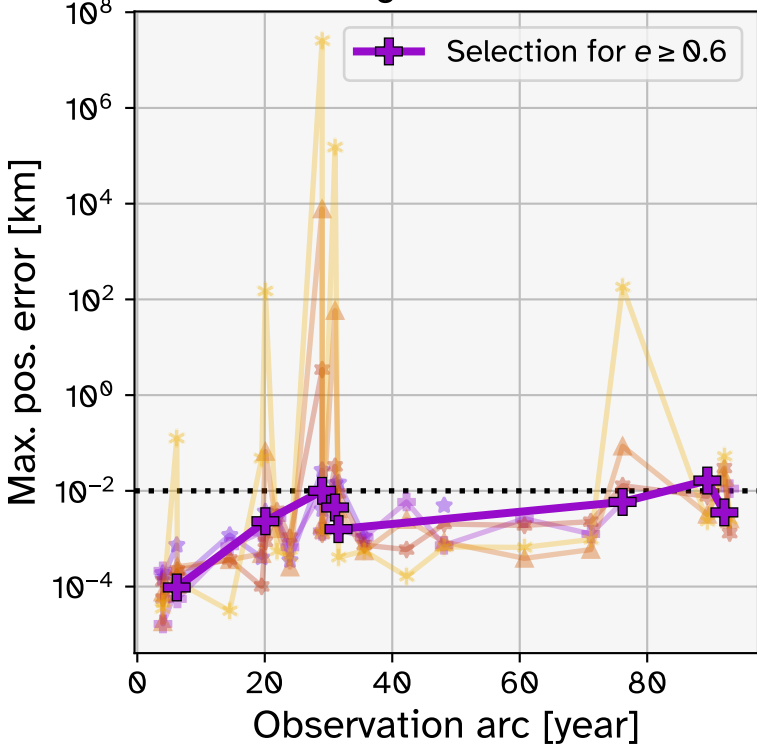
Integrator: RK10
