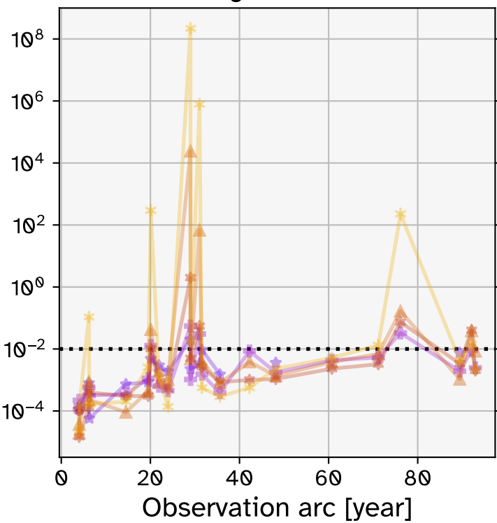
Integrator: RK12
