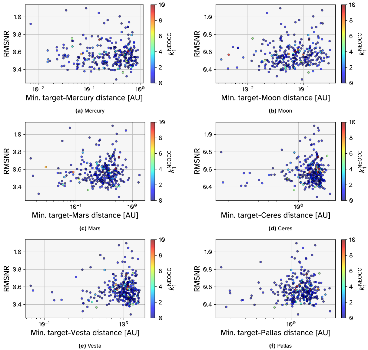
Figure A.1: Distributions of RMSNR of the Tudat estimations against the minimum distance between the target body and the inner planets (except Venus and Earth, whose figures were shown in Subsection 4.3.4, see Figure 4.41) and the three most massive bodies in the main asteroid belt. The points are coloured according to their value of k_1^{\text{NEOCC}} .
