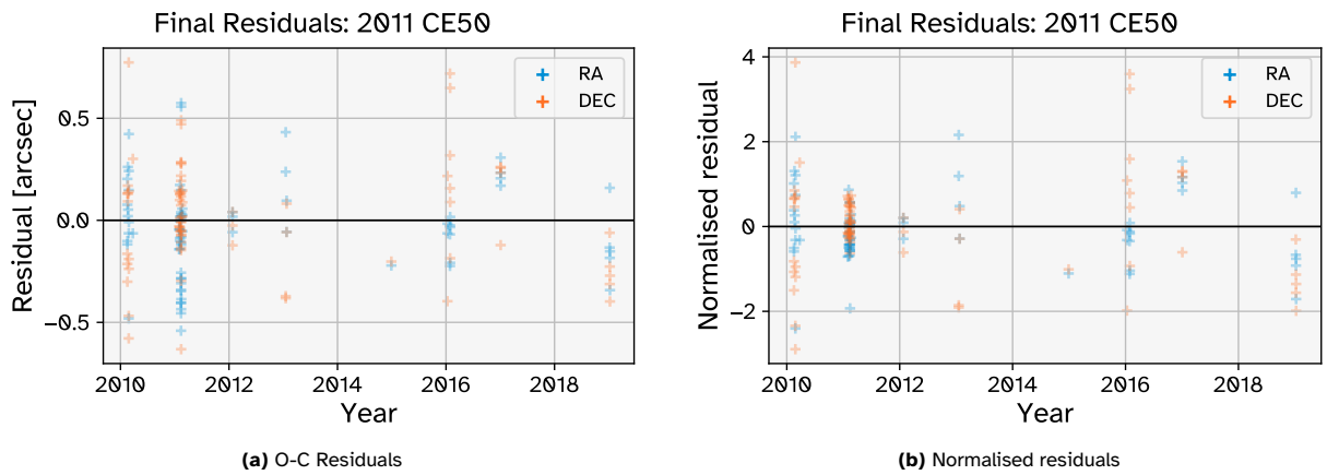
Figure 4.11: Residuals for the best iteration of the estimation of asteroid 2011 CE 50 .
