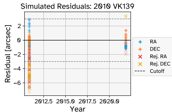
Figure 3.17: Simulated RA-DEC residuals for asteroid 2010 VK 139 , for which a particularly high proportion of observations were rejected. Accepted observations are marked with '+'. Rejected observations are marked with 'X'.
