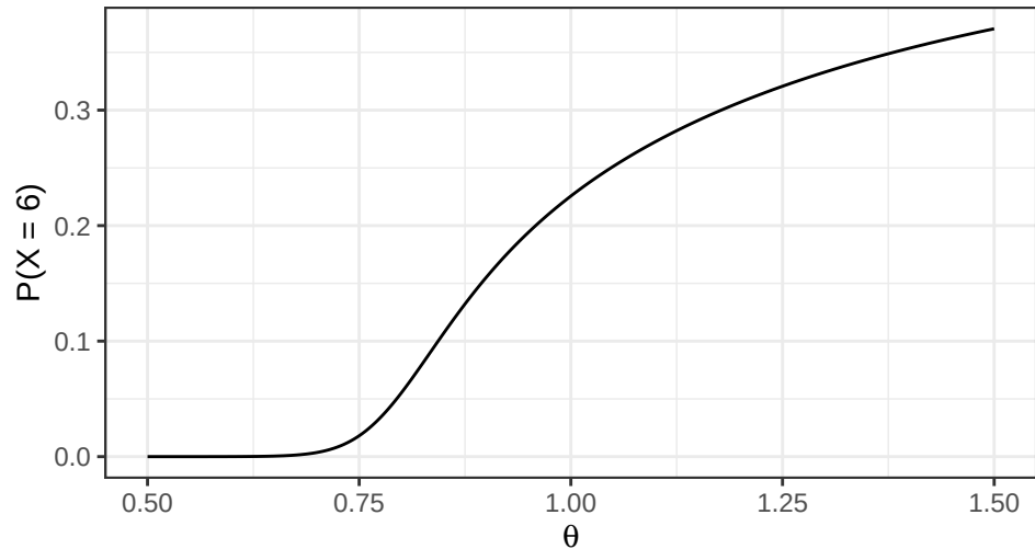
P(X = 6) vs. \theta
