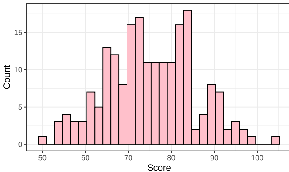
Figure 4: Histogram Plot
