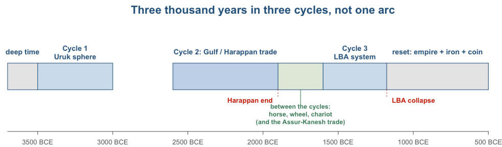
Figure 1.8. Three thousand years in three cycles, not one arc: an early Uruk world system rises and contracts, the Gulf trade the Harappans ran follows and ends with their cities c.1900 BCE, and after a gap that the steppe technologies carry, the Late Bronze Age system rises and collapses c.1177 BCE, before the reset by 500 BCE. Drawn to a linear time axis, so the long interval between cycles two and three is real time rather than spacing. Author's schematic.
