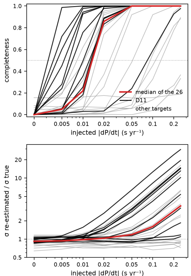
Fig. 4. A secular term through the estimator of the chain (Sect. 5.2.5). Top: completeness — the fraction of injected terms passing the curvature test and the adversarial gate with the bars re-estimated inside the simulation — against the injected |dP/dt| , one curve per target (black: D11; grey: the others; red: the median of the 26; the point at 0 is the false-alarm rate). Bottom: the suppression factor, \sigma(dP/dt) with the re-estimated bars over \sigma with the true bars, on the same grid. Both are properties of the 4–7-epoch design, not of the complete TESS block of Sect. 5.5.
