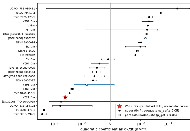
Fig. 1. Quadratic coefficients dP/dt of the 26 targets with 1\sigma bars, ordered by value; the three flagged targets ( p_{\text{gof}} < 0.05 ) are shown open, and V527 Dra is marked.
