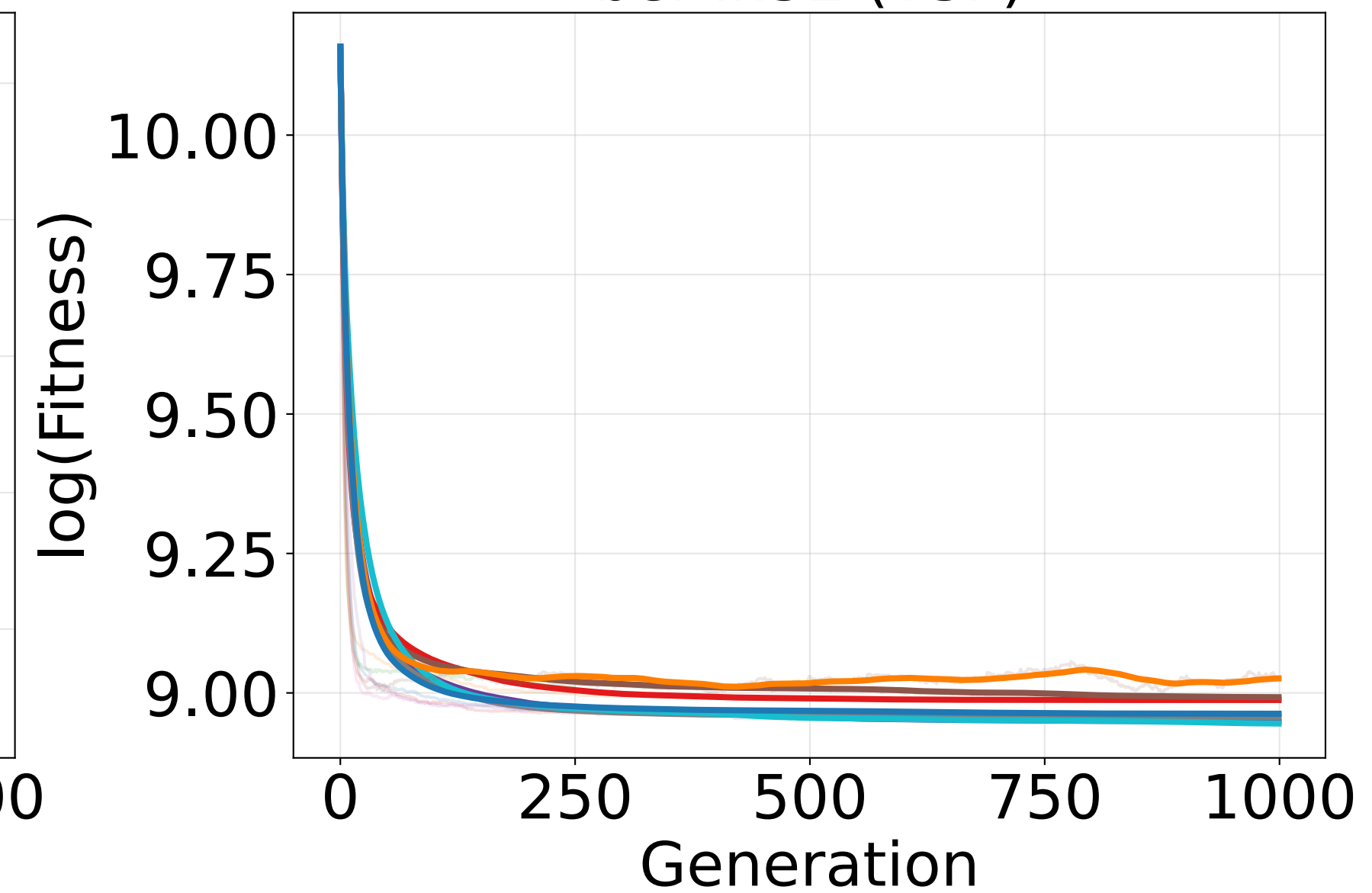
berlin52 (TSP)
