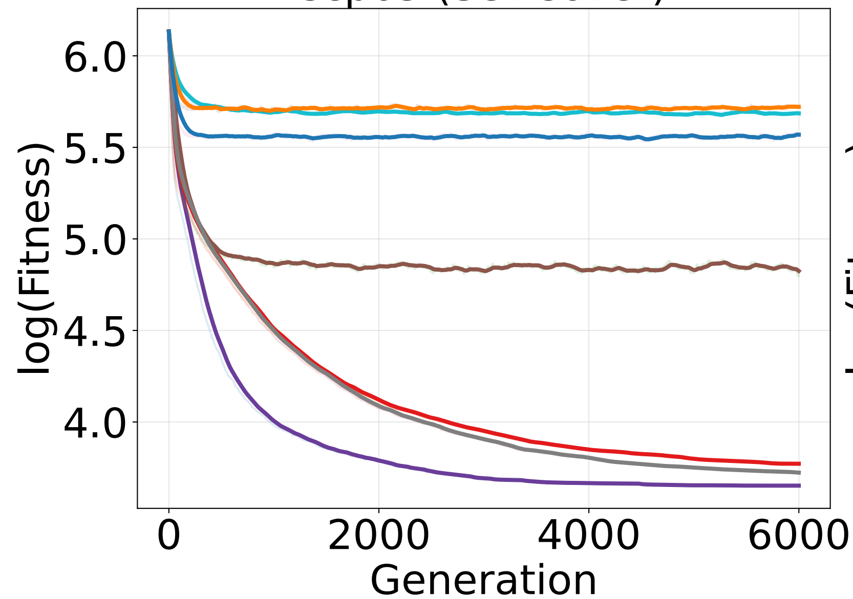
scp65 (Set Cover)
