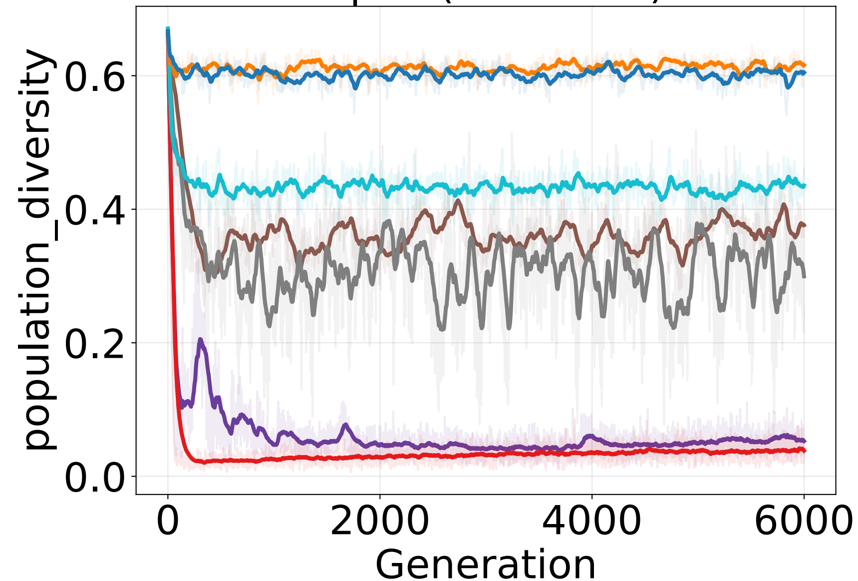
scp65 (Set Cover)
