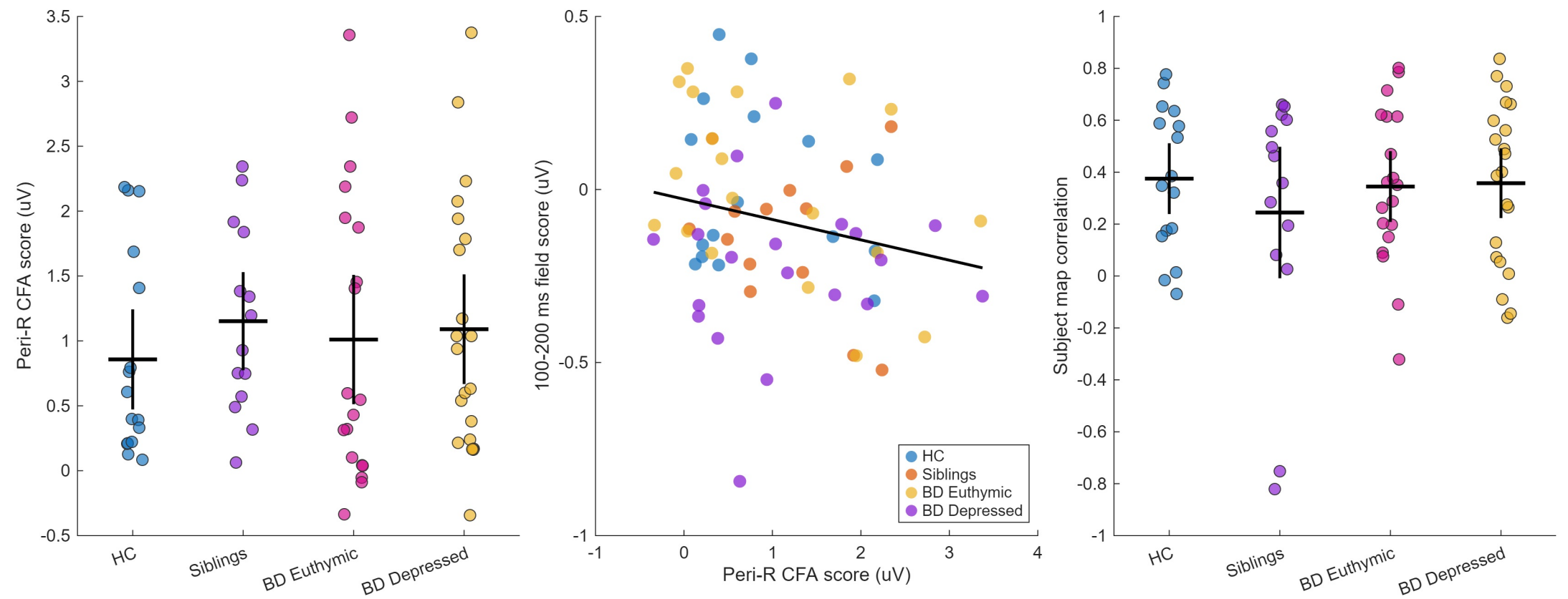
Figure 4. Peri-R artifact control and primary 100-200 ms robustness analyses
