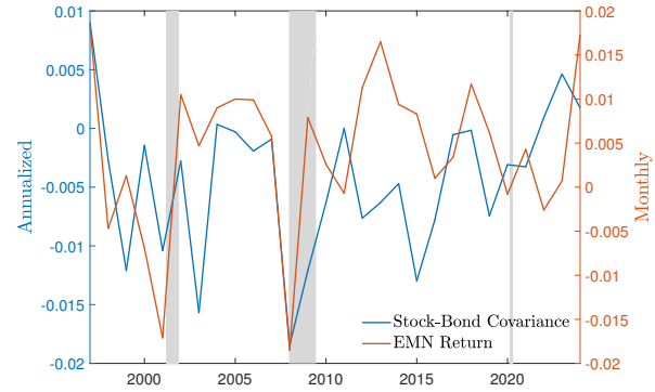
(b) Annual Covariance and EMN Returns
