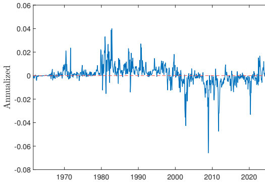
(a) Monthly Stock-Bond Covariance
