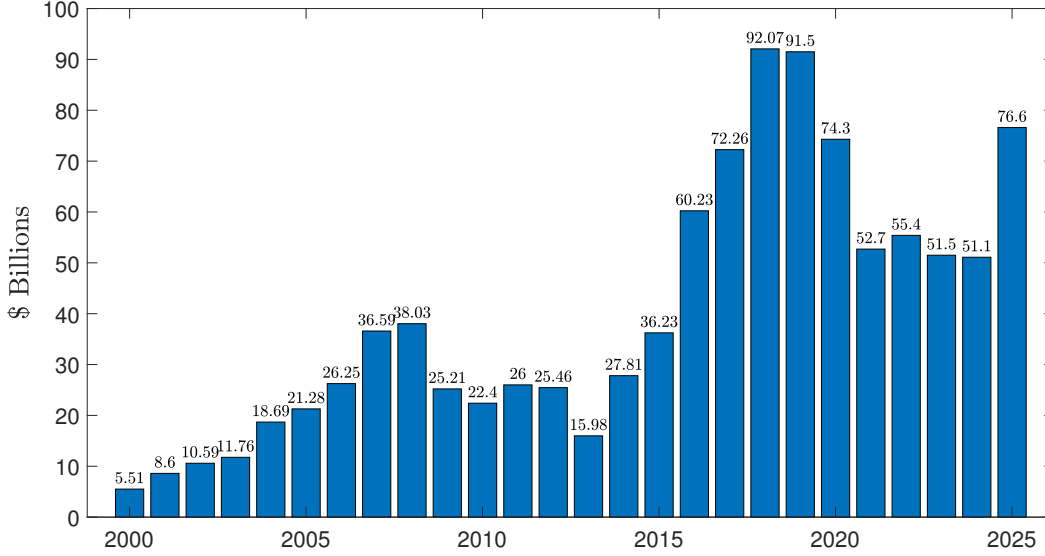
Figure. D.4. Asset Under Management of Equity Market Neutral Hedge Funds
