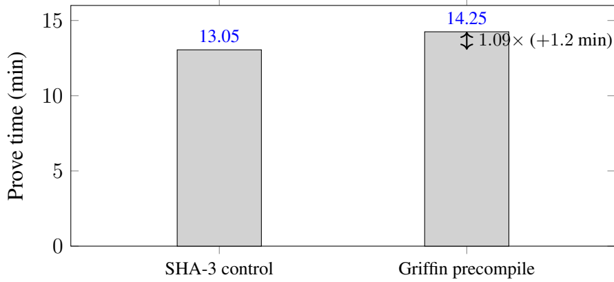
Figure 4: Prove time of the two SP1 arms that share the same PLUM verification at matched \lambda = 80 (M5 Pro 24 GB, linear scale, n = 3 means). The bespoke Griffin precompile (14.25 min) is slower than the SHA-3 control (13.05 min): a 1.09\times wall-clock inversion ( 1.13\times in cycles), the falsified speedup. The precompile-free baseline does not complete (DNF, OOM at \approx 1m45s ); RISC Zero’s sys_bigint route completes in 6 h 19 m (Table 2).
