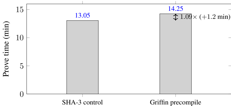
Figure 4: Prove time of the two SP1 arms sharing the same PLUM verification ( \lambda = 80 , n = 3 ). The Griffin precompile is slower than the SHA-3 control—the inversion; the no-precompile baseline does not complete.
