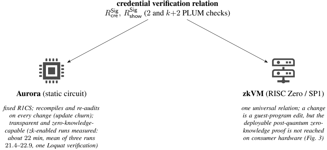
Figure 1: One relation, two outer provers. The same credential verification relation is proved either by a static Aurora circuit (the BDEC baseline) or by a general-purpose zkVM (this thesis)—alternatives, not composed. The figure also locates the deployability wall: Aurora reaches an accepted post-quantum zero-knowledge proof of the Loquat building block, whereas the zkVM does not on consumer hardware.
