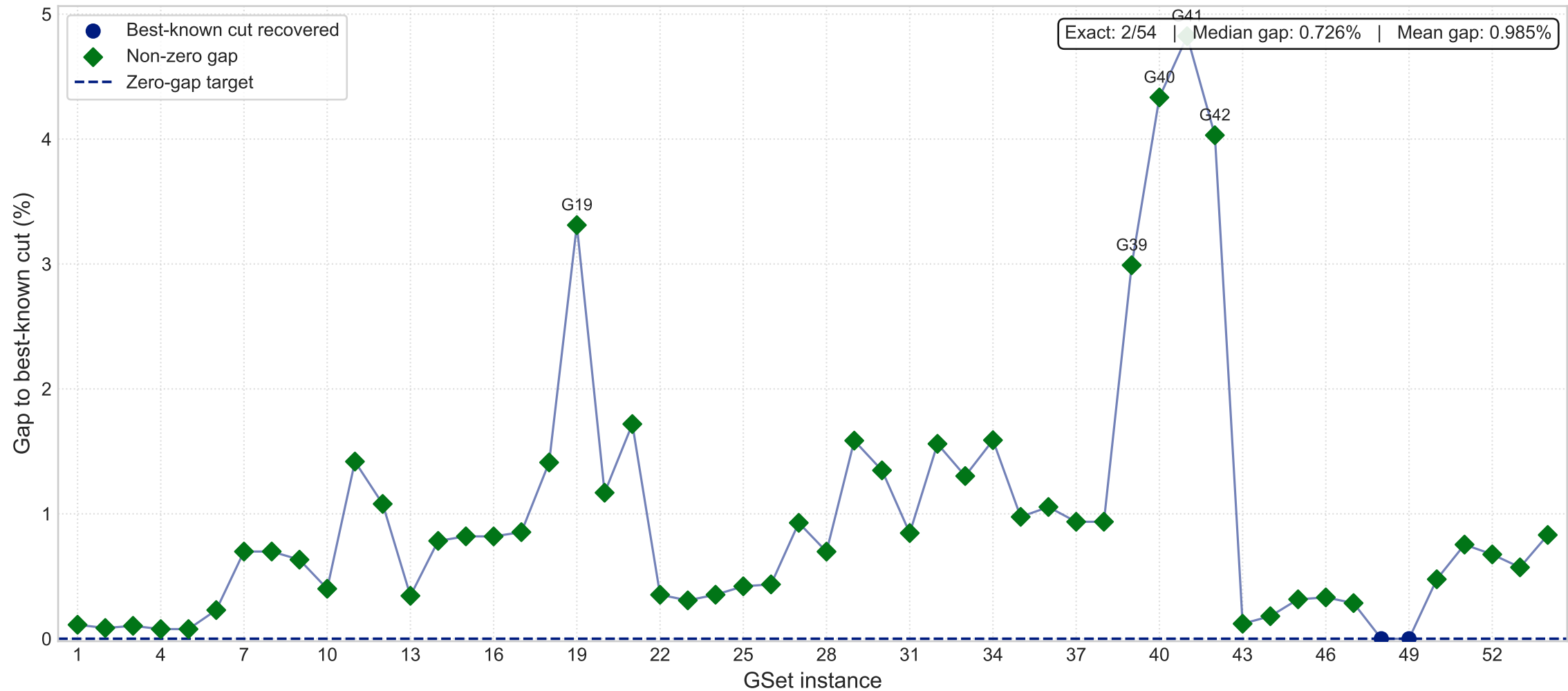
Initial QeFEM V1 Performance on GSet
