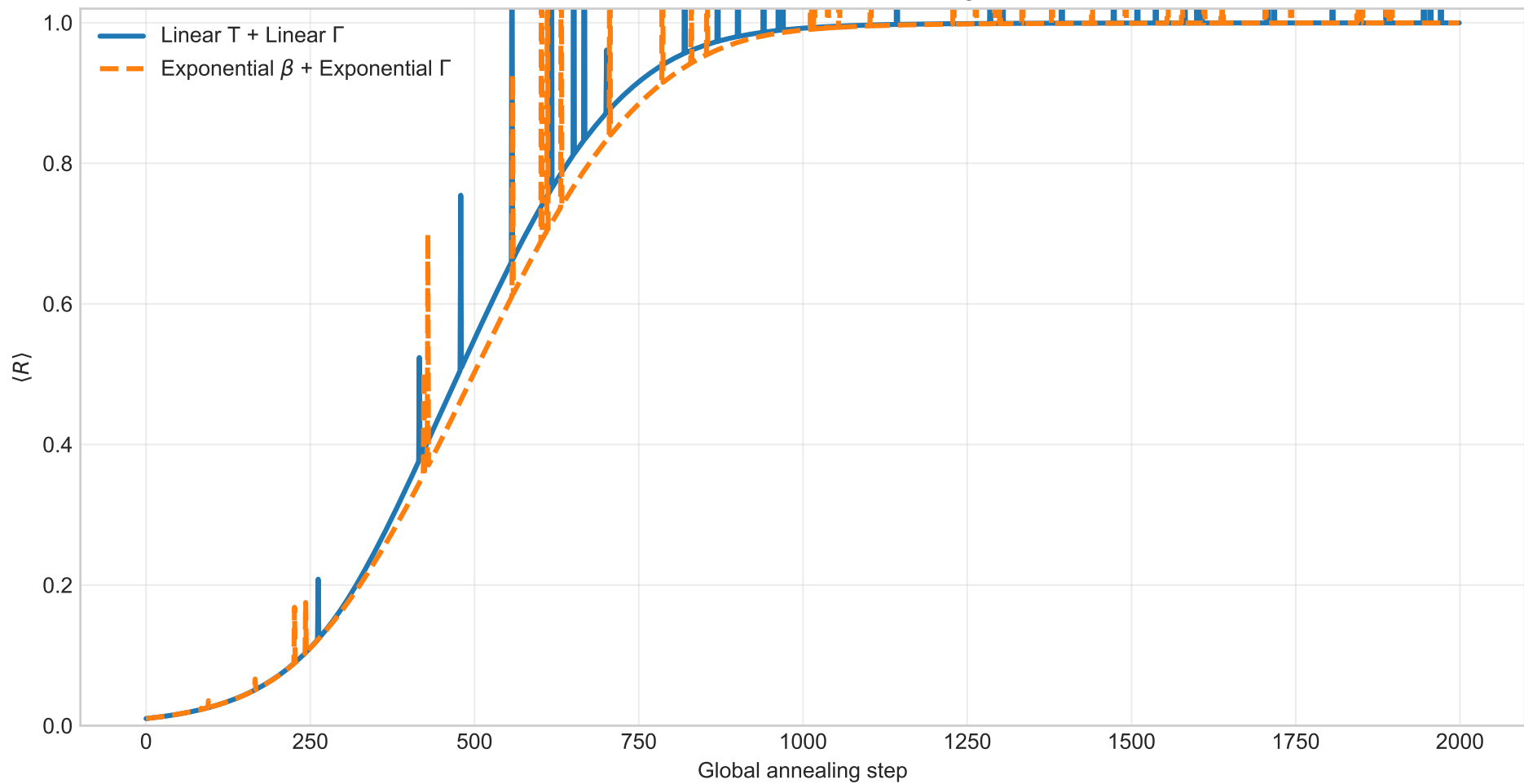
G4: Evolution of Mean Bloch Length R
