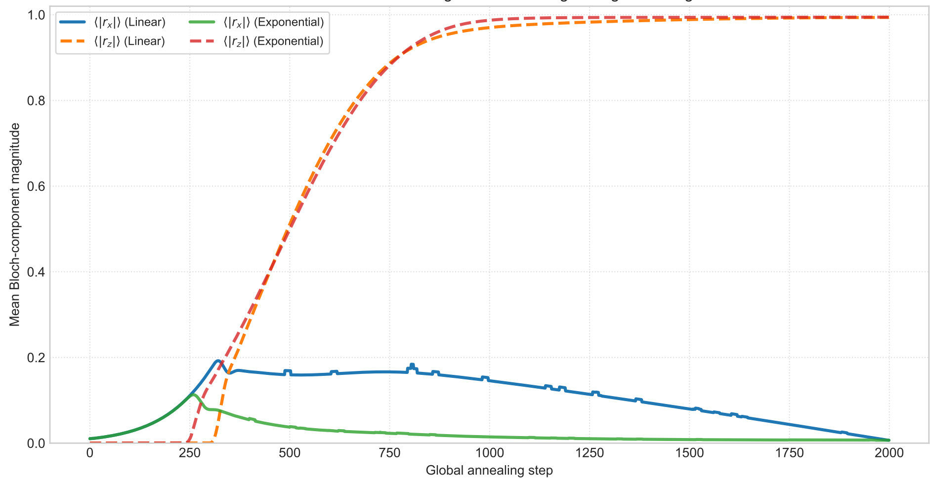
G4: Transverse-to-Longitudinal Ordering During Annealing
