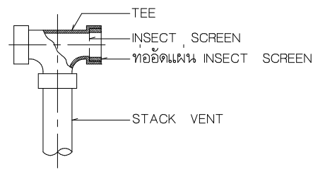
VENT TERMINAL ( VT ) NOT TO SCALE
