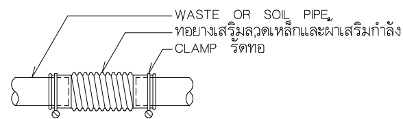
DRAINAGE FLEXIBLE JOINT ( DF ) NOT TO SCALE
