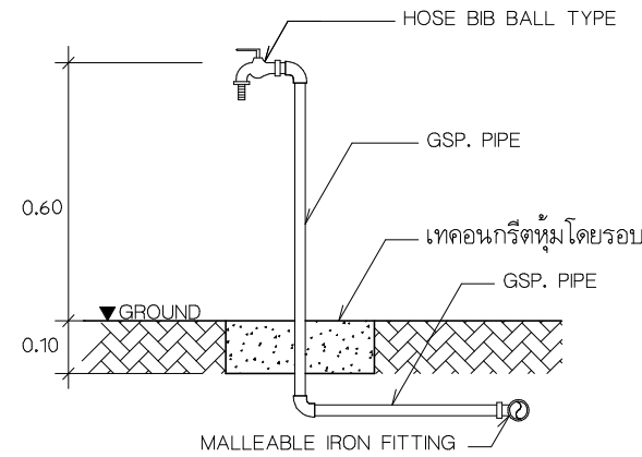
HOSE BIB ( HB ) NOT TO SCALE
