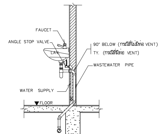
LAVATORY (LAV.) NOT TO SCALE
