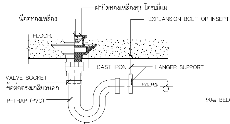
FLOOR DRAIN 2 ( FD ) NOT TO SCALE
