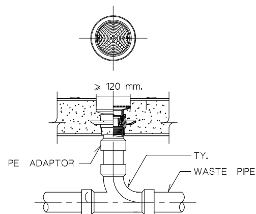
FLOOR DRAIN 1 ( FD ) NOT TO SCALE
