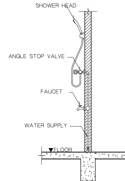
HAND SHOWER NOT TO SCALE
