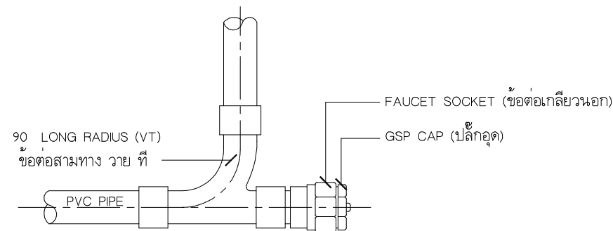
CLEANOUT NOT TO SCALE
