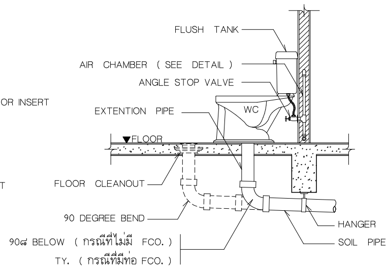
WATER CLOSET (WC.) NOT TO SCALE
