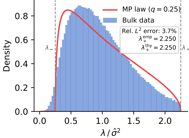
FIG. 1. Bulk eigenvalue density histogram of aggregated normalized bulk eigenvalues across all windows for PETR4, M5 frequency. Orange curve: theoretical MP density (Eq. ??) with q = 0.25 , \hat{\sigma}^2 = 1 . Vertical dashed lines: theoretical \lambda_{\pm} . Inset: relative L^2 error for all assets in Table ??.
