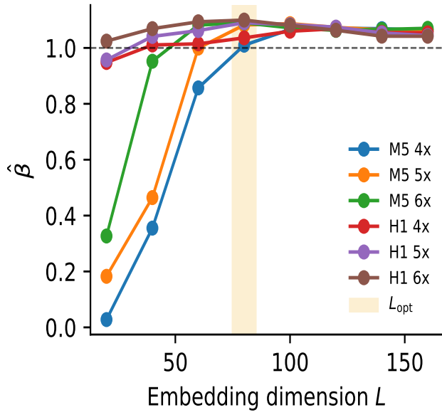
FIG. 3. Intrinsic embedding dimension. Diffusive exponent \hat{\beta} vs. embedding dimension L for M5 and H1 data, with n = W/L \in \{4, 5, 6\} . Both timescales yield L_{\text{opt}} \approx 80 regardless of n . Shaded region: L_{\text{opt}} \in [75, 85] .
