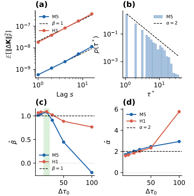
FIG. 2. Universal exponents, data from PETR4. (a) Log-log plot of \mathbb{E}[\|\Delta\mathbf{K}\|_F^2] vs. temporal lag at M5 and H1 timescales. Dashed: slope \beta = 1 . (b) Histogram of inter-regime intervals \tau^* frequencies on log-log scale for M5 timescale. Dashed: slope \alpha = 2 . (c) and (d) Estimated \beta (left) and \alpha (right) as functions of \Delta\tau_0 (candles) for M5 and H1 timescales. Both exponents converge to (1, 2) in the range \Delta\tau_0 \lesssim 30 . The shaded region is the optimal choice for observation step \Delta\tau_{\text{opt}} \approx 20 .
