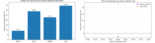
Figure 2: Left: fixed non-native source layers strongly degrade T15 phoneme decoding relative to native-day decoding. Right: small learned calibration improves over the fixed-middle source but remains far from native-day decoding.
