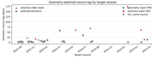
Figure 5: Geometry-selected older sources are meaningful candidates but not reliable standalone decisions at K = 20 . Left: most target sessions select the immediately previous session, but several jump to older stored input states. Right: geometry-selected sources are closer in covariance distance by construction, but lower geometry distance does not always translate to lower PER. Green points indicate cases where the geometry-selected source outperforms previous; red points indicate cases where previous remains better.
