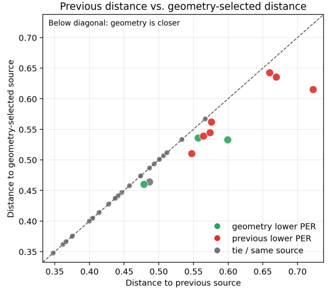
Figure 5: Geometry-selected older sources are meaningful candidates but not reliable standalone decisions at K = 20 . Left: most target sessions select the immediately previous session, but several jump to older stored input states. Right: geometry-selected sources are closer in covariance distance by construction, but lower geometry distance does not always translate to lower PER. Green points indicate cases where the geometry-selected source outperforms previous; red points indicate cases where previous remains better.
