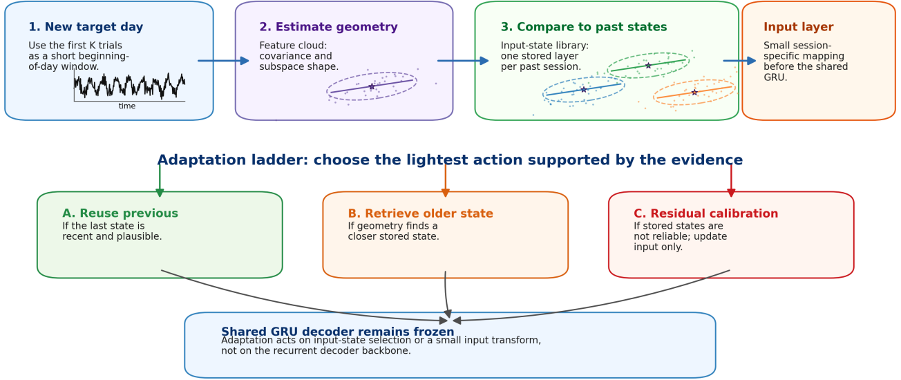
Figure 1: Recency-aware input-state selection for cross-session BCI drift. For a new target session, the first K trials are used to estimate neural feature geometry. Each session is represented as a cloud of neural feature vectors, summarized by covariance and subspace statistics. The target geometry is compared to a library of past input states. The system first reuses the previous input layer when it is recent and plausible; otherwise, geometry can retrieve an older candidate state. If no stored state is reliable, only the input layer is lightly calibrated while the shared GRU decoder remains frozen.
