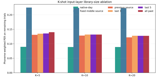
Figure 3: Library-size ablation. A small recent library approaches all-past geometry selection, but previous-session recency remains the strongest aggregate policy under the current covariance-nearest rule.
