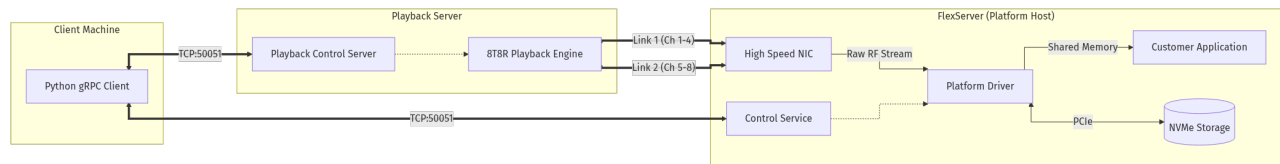
Figure 2: XRComm 8T8R Playback Platform Topology
