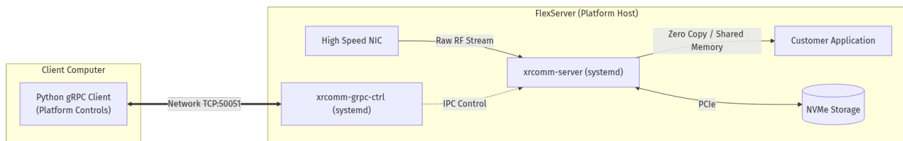
Figure 1: XRComm FCS 8T8R Platform Topology
