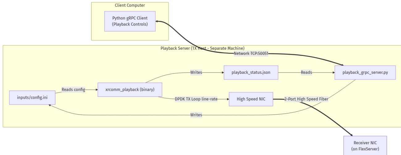
Figure 2: XRComm 8T8R Playback Platform Topology
