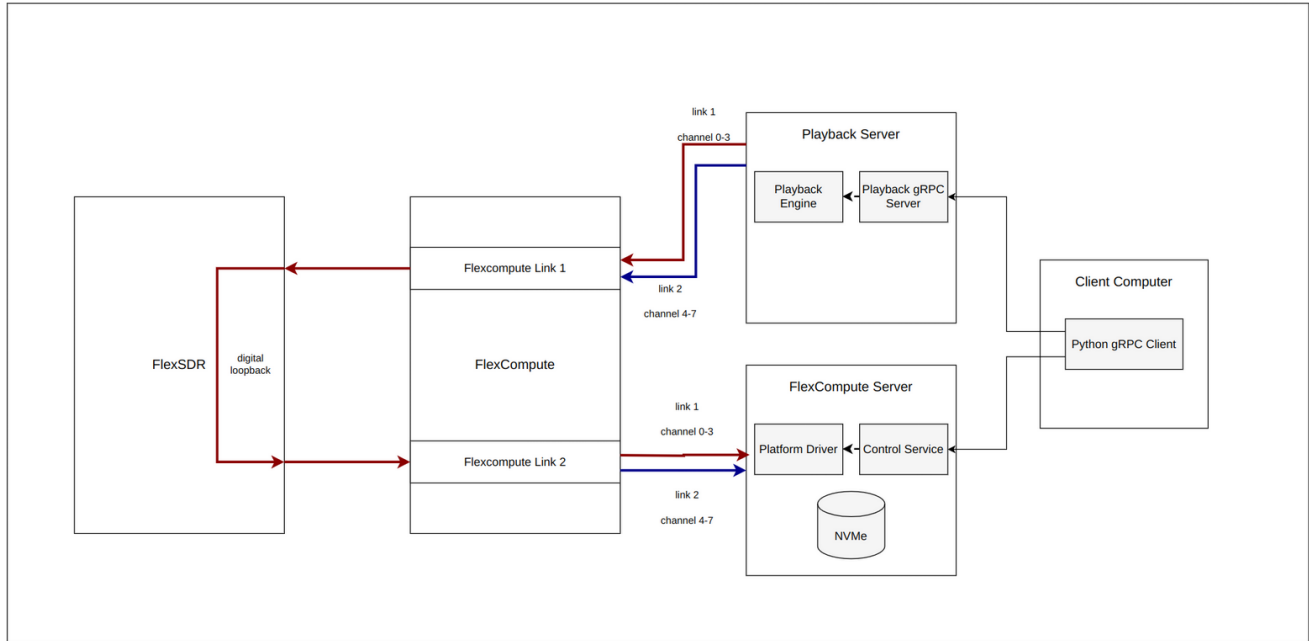
Figure 1: XRComm FCS 8T8R Platform Topology
