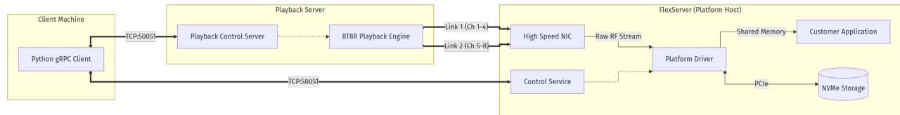
Figure 1: XRComm FCS 8T8R Platform Topology
