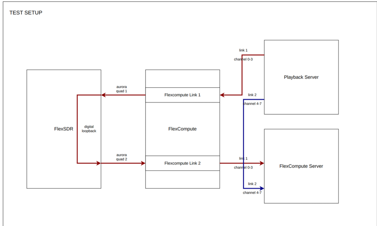
Figure 1: XRComm FCS 8T8R Platform Topology
