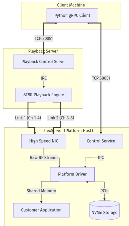
Figure 1: XRComm FCS 8T8R Platform Topology
