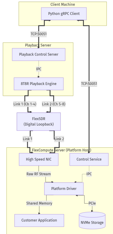
Figure 1: XRComm FCS 8T8R Platform Topology
