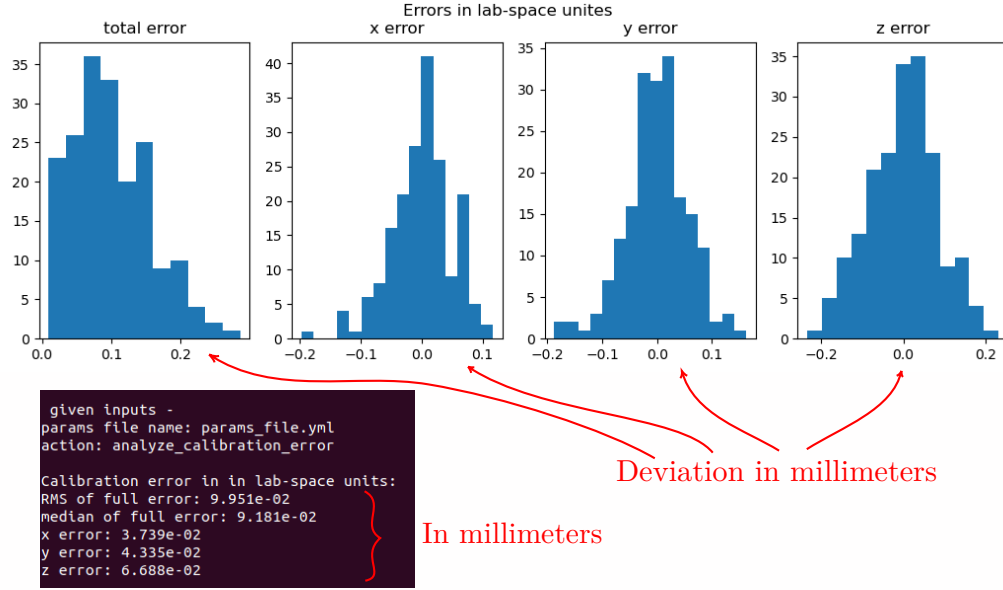
Figure 7: Example results of the calibration error analysis. In this experiment, the lower bound for the uncertainty for position measurements based on the RMS deviation value was approximately 100\ \mu\text{m} , with the largest deviations in the z direction.
