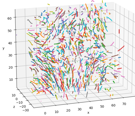
Figure 16: Trajectory segments plotted using the workflow plot_trajectories command. A 30 frames long segment is shown from a turbulent flow dataset taken from Ref. [8].
