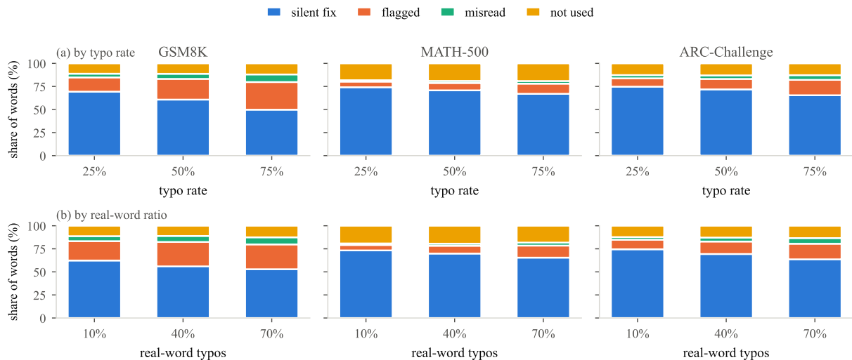
Figure 4: Word-level repair behaviour. Word-level repair behavior. How every corrupted word is handled in the reasoning trace. (a) against the typo rate, pooled over real-word ratios. (b) against the real-word ratio, pooled over typo rates. Section 5.3 claims a trend on both axes and both are present: silent Silent fixing gives way to explicit flagging and to outright misreading as either knob is turned up the typo rate or the real-word ratio increases, while the share of words never referred to at all stays roughly constant. Per-configuration values are in Table A5.
