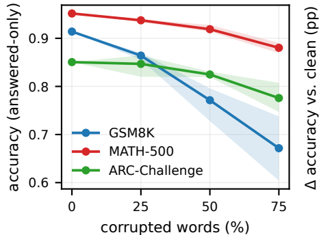
(a) absolute accuracy
