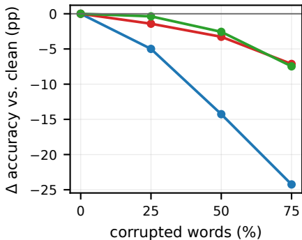
(b) accuracy tax
