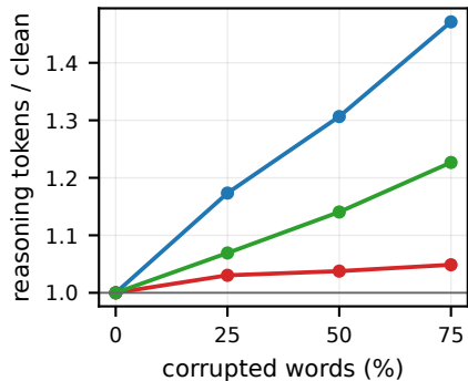
(c) reasoning-length tax
