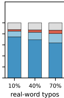
ARC-Challenge
