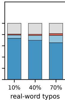
MATH-500
