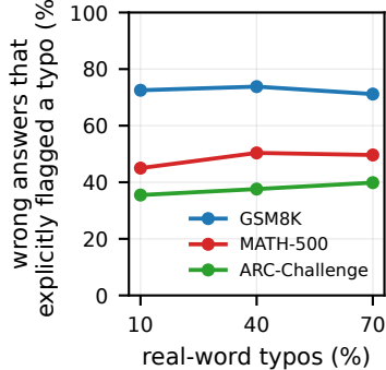
silent-failure test
