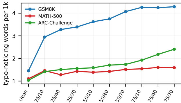
(b) explicit typo talk
