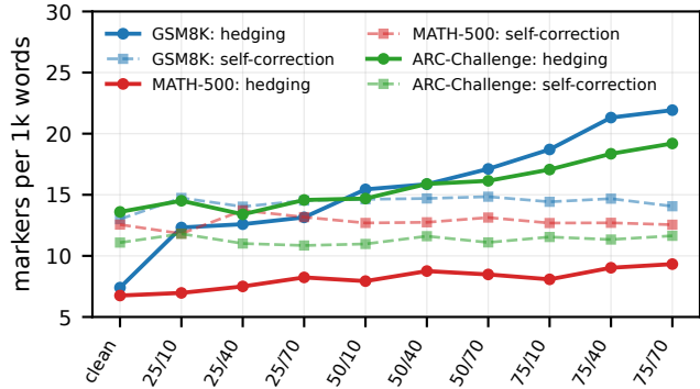
(a) hedging rises, self-correction does not
