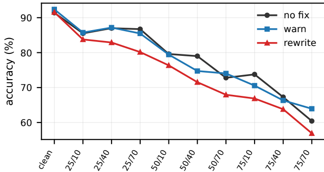
(a) GSM8K accuracy under each fix
