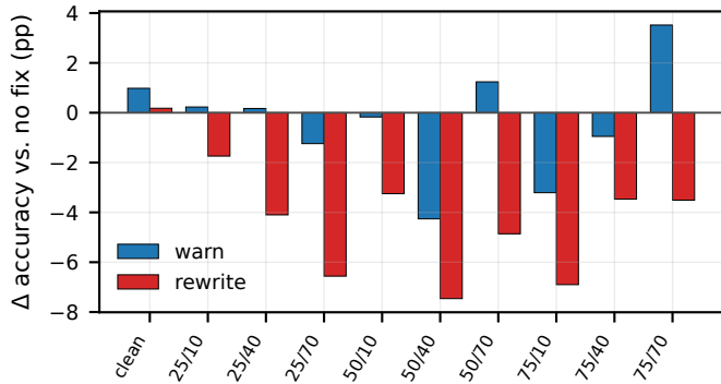
(b) neither fix recovers the loss
