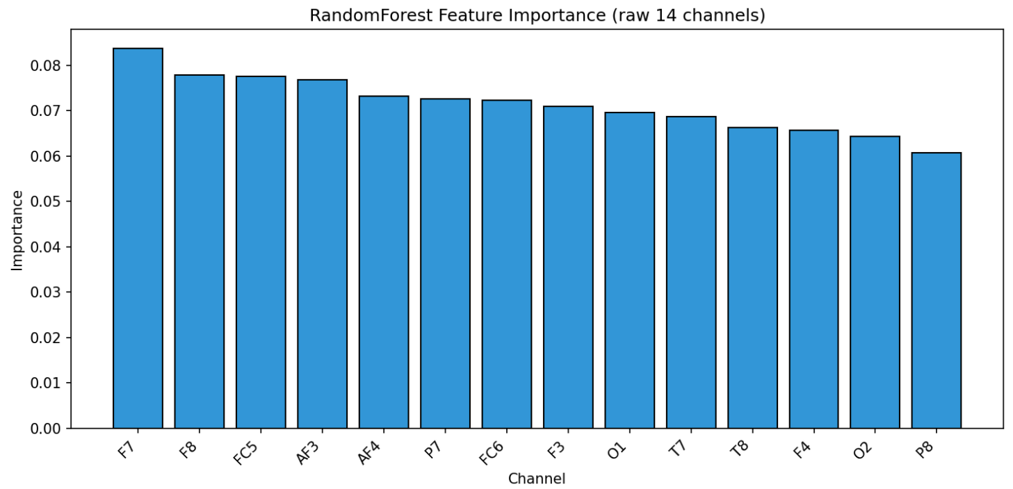
Feature Importance (RandomForest — 70/15/15 training partition):
