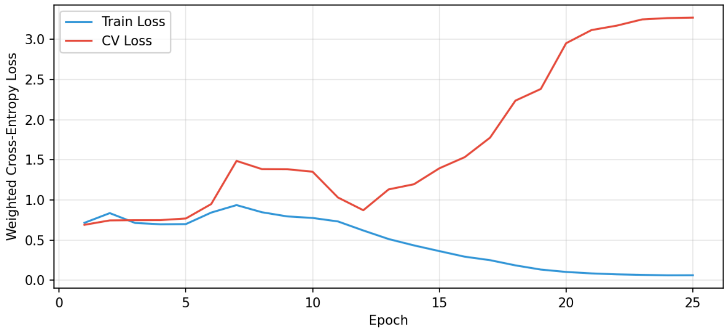
LSTM — Train vs CV Loss Curve
