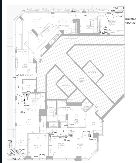
HVAC system design for Apt #21LMZ
