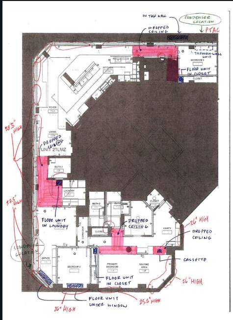
Preliminary survey for Design and Calculations
