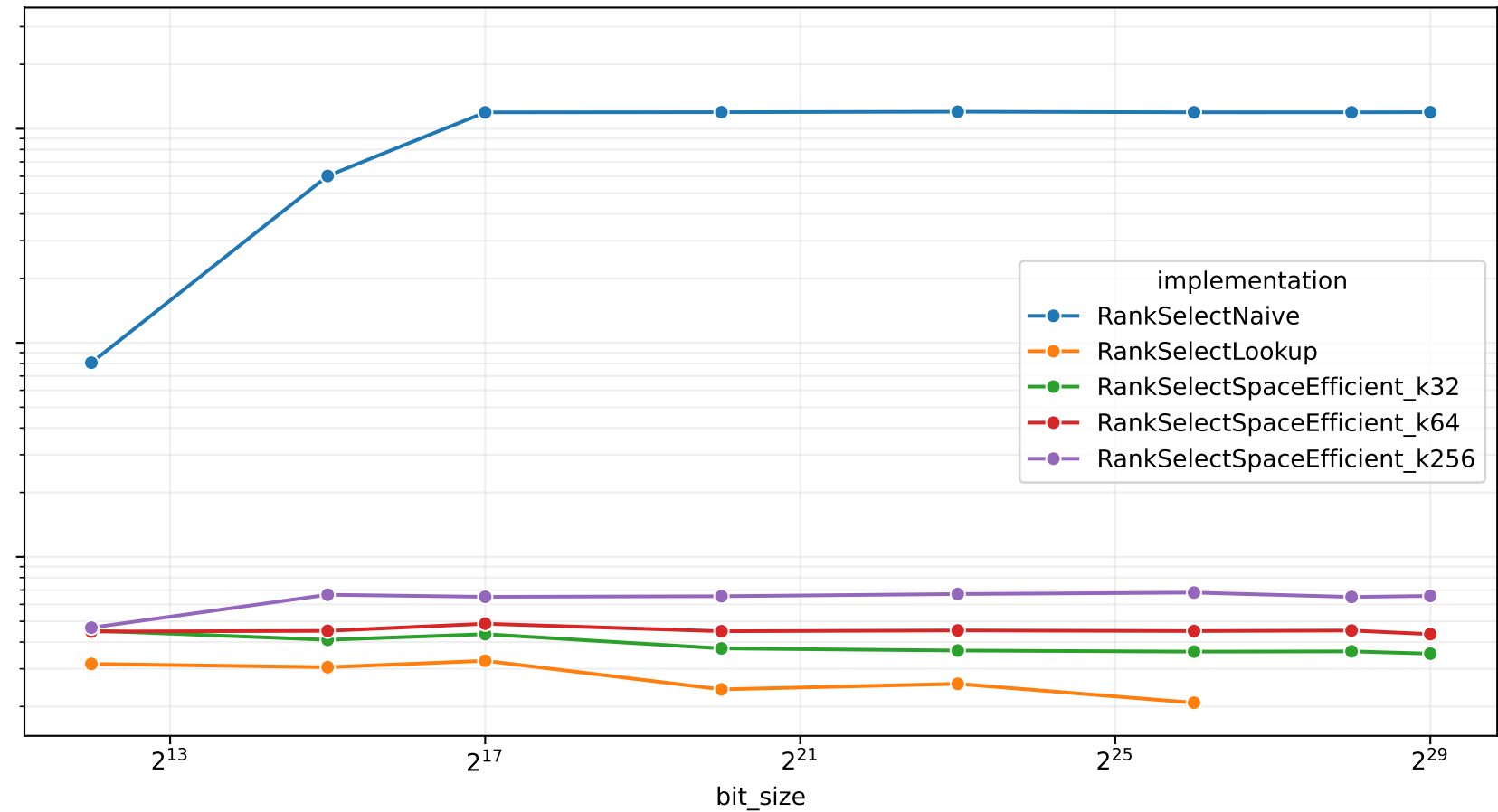
Rank operations as a function of n - With queries Sequential
