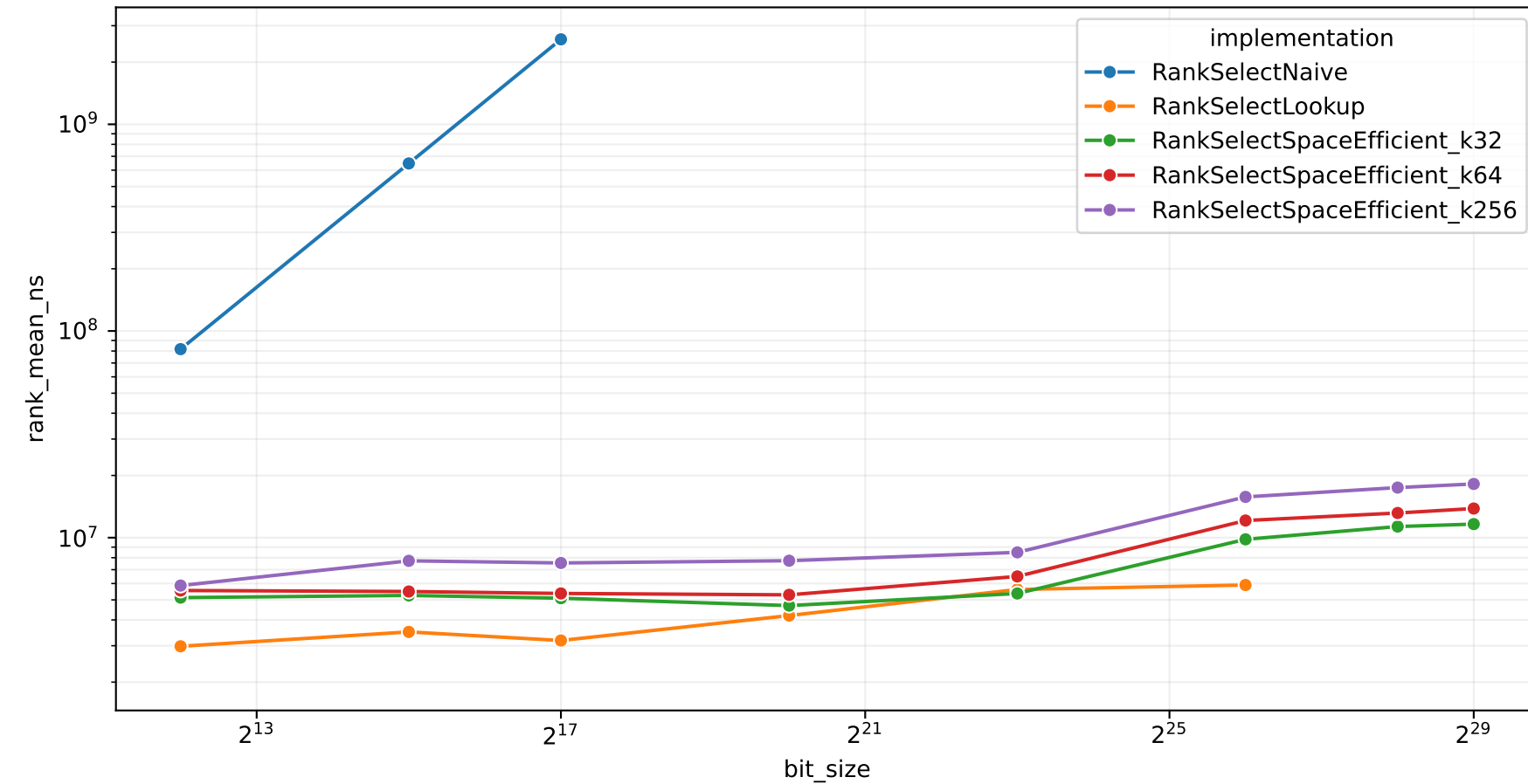
Rank operations as a function of n - With queries Random Uniform Data
