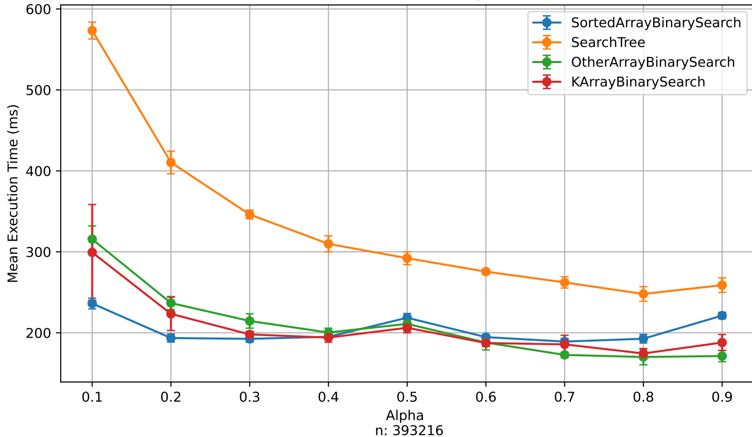
Execution Time vs Alpha
