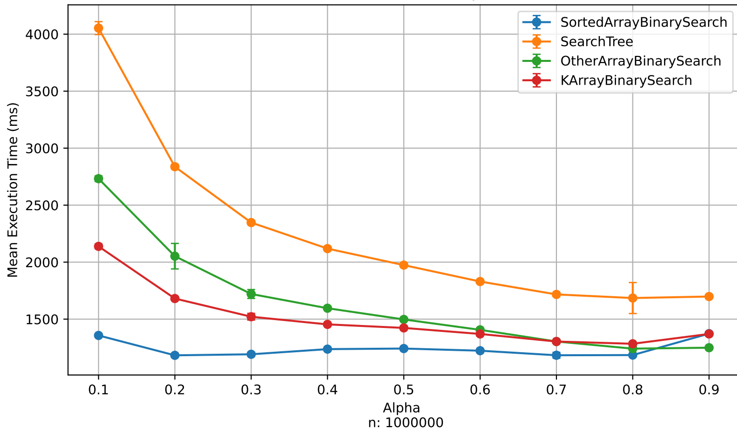
Execution Time vs Alpha
