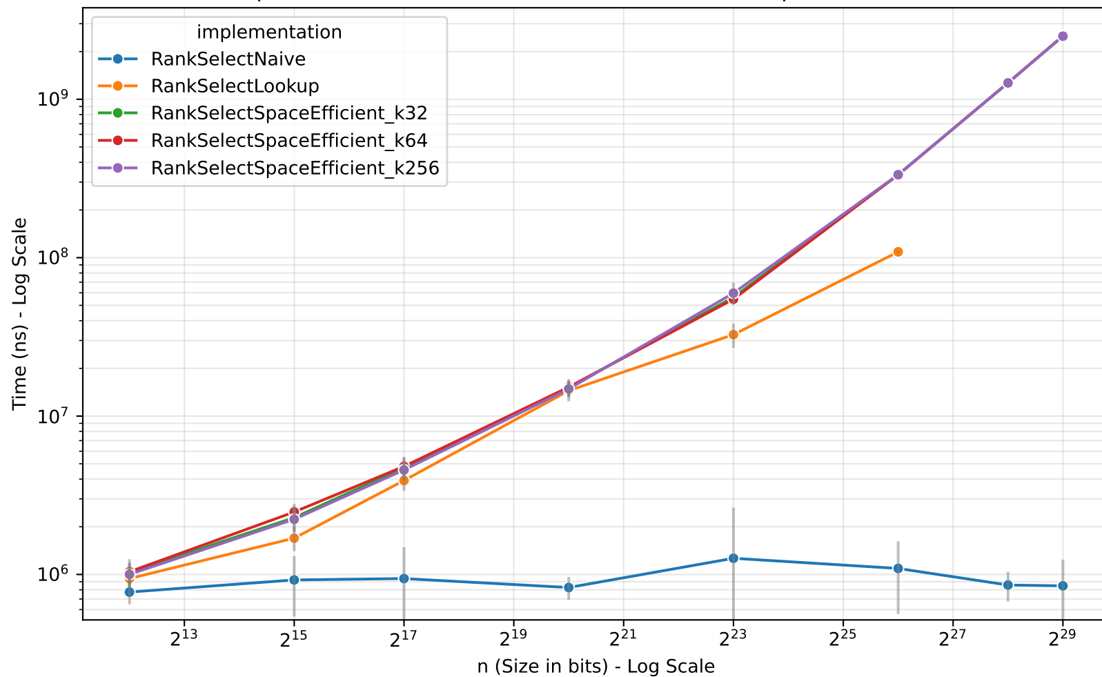
Implementation Build Time as a Function of n (Sequential Queries)
