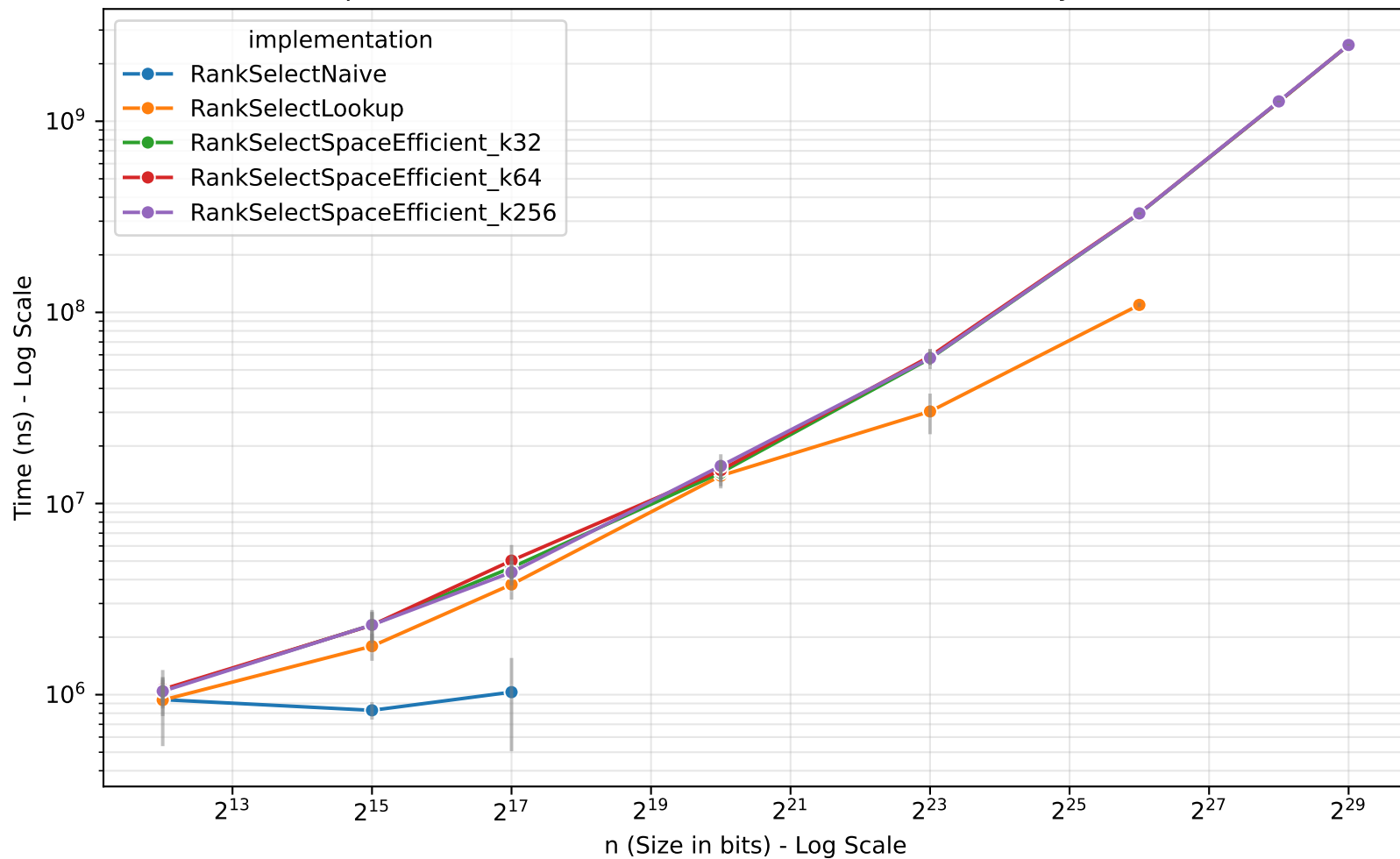
Implementation Build Time as a Function of n (Locality Queries)
