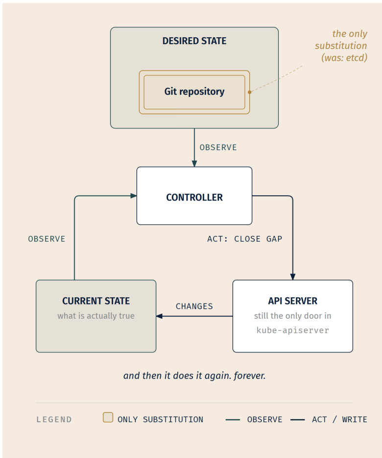
Figure 15.7 — The control loop, pointed at a repository. Lay this beside Chapter 3's control-loop figure and the point is that it is the same loop. The controller sits in the same place, the API server is still the only door in, and the arrows run in the same directions. One box changed contents.
