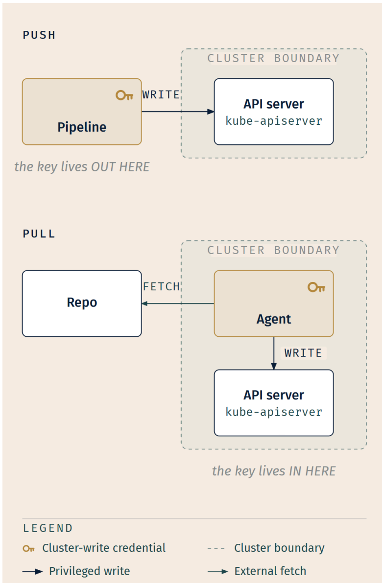
Figure 15.3 — Push and pull, mirrored. The cluster boundary is the same line in both panels and the arrow is the only thing that reverses. Watch the key: in push it sits outside the boundary, in a system the cluster does not control. In pull it sits inside, in a Pod the cluster does control. Everything else in this section is a consequence of that one difference.
