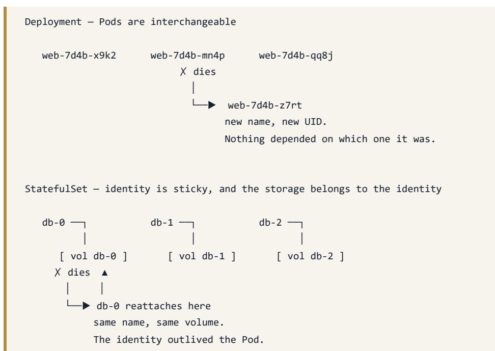
Figure 6.4 — the storage belongs to the identity, not to the Pod. Look at the lower row carefully. The volume is not drawn attached to a Pod; it is drawn
