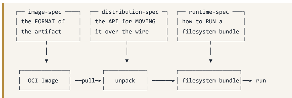
Figure 2-4. Specifications on top, artifact lifecycle underneath, one column each. What to notice: nothing in this figure is Kubernetes. Compare it against Figure 2-3. Those are two different planes, and the next callout is about exactly that.
