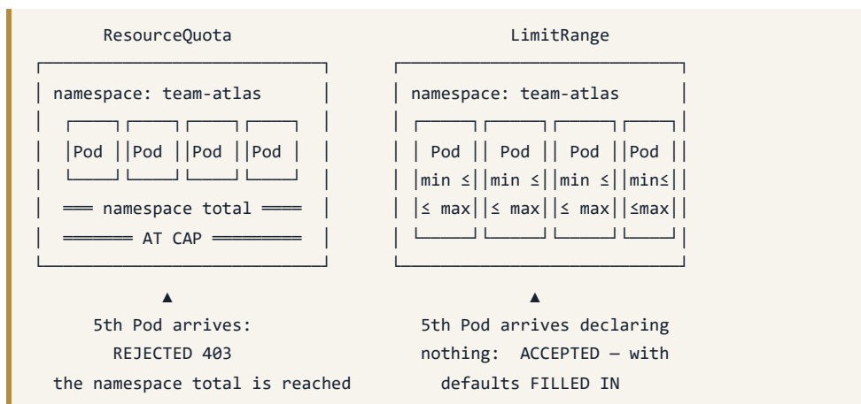
Figure 8.3 — Both mechanisms live inside one namespace; the boundary is the same on each side and is not the discrimination. What differs is what is being counted and how it fails. On the left, one aggregate total for the namespace, and a fifth Pod rejected at the cap. On the right, per-object
