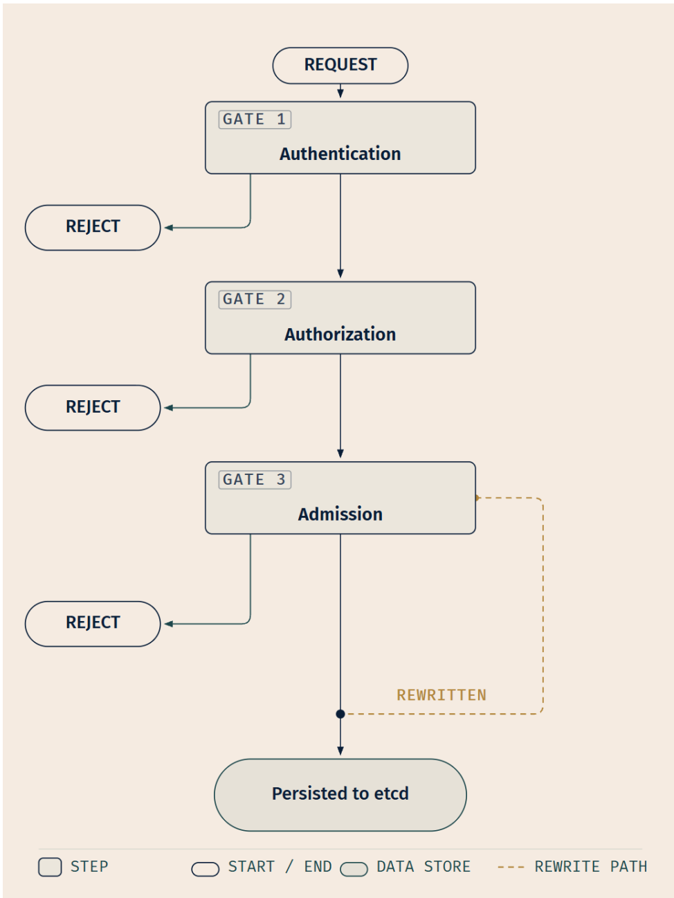
Figure 8.2 — What to notice is the fourth arrow. Gates one and two have one way out other than forward: refusal. Gate three has two. It can refuse, or it can alter the request and let the altered version continue. The three questions, in order, are: who are you , may you do this , and should this, as written, be allowed .
