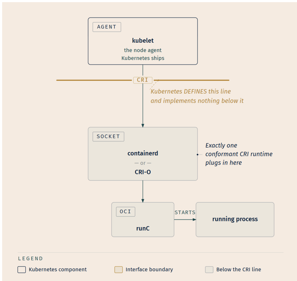
Figure 2-3. What to notice is the socket, not the boxes. containerd and CRI-O are not two parallel paths through the system; they are two things that fit
