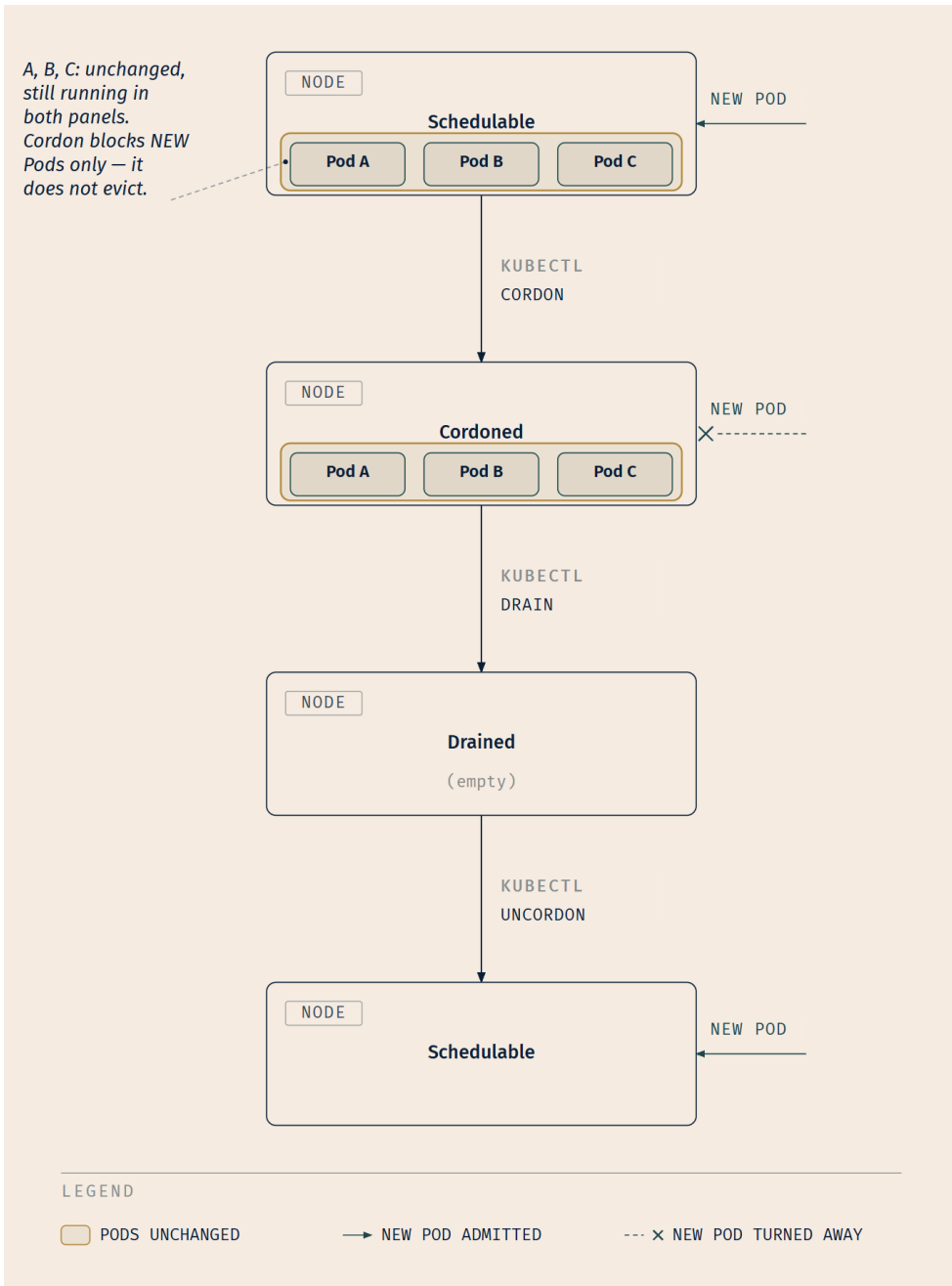
Figure 8.4 — What to notice is what does not change between the first two panels. The three Pods aboard the cordoned node are still running, still serving, still entirely unaffected. Only the arriving Pod's fate differs. The node does not empty until drain.
