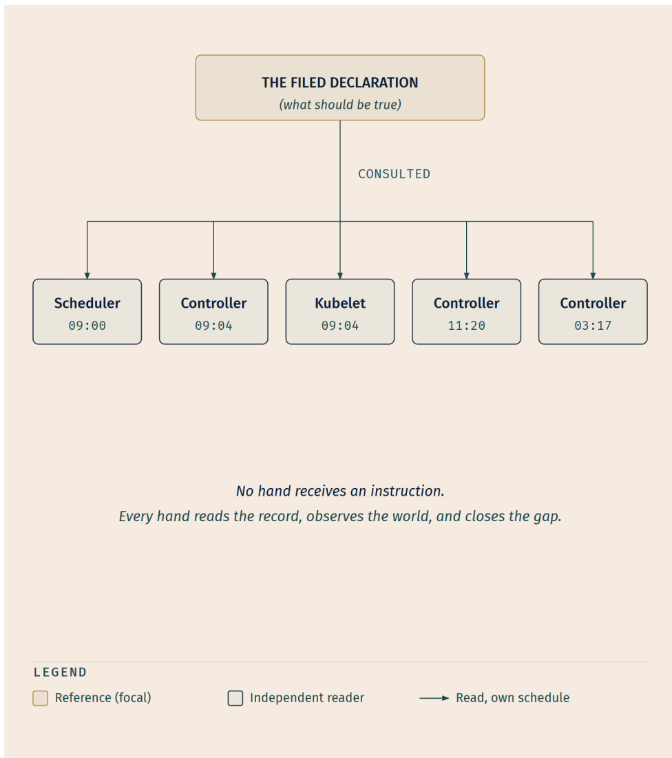
Figure: the record outranks the moment it was written. Nothing in this figure is a command being passed down a chain; every arrow is a reading.
