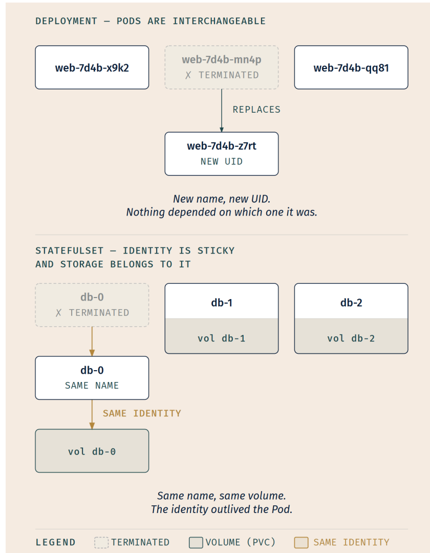
Figure 6.4 — the storage belongs to the identity, not to the Pod. Look at the lower row carefully. The volume is not drawn attached to a Pod; it is drawn attached to db-0 , which is a slot that Pods pass through. That is the claim, and Chapter 11 is where it gets completed.
