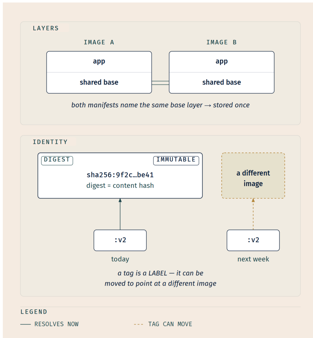
Figure 2-2. Two ideas in one frame, because §3 depends on the right half. What to notice: the dashed arrow. The tag :v2 is attached to the image, not part of it, and an attachment can be re-attached.
