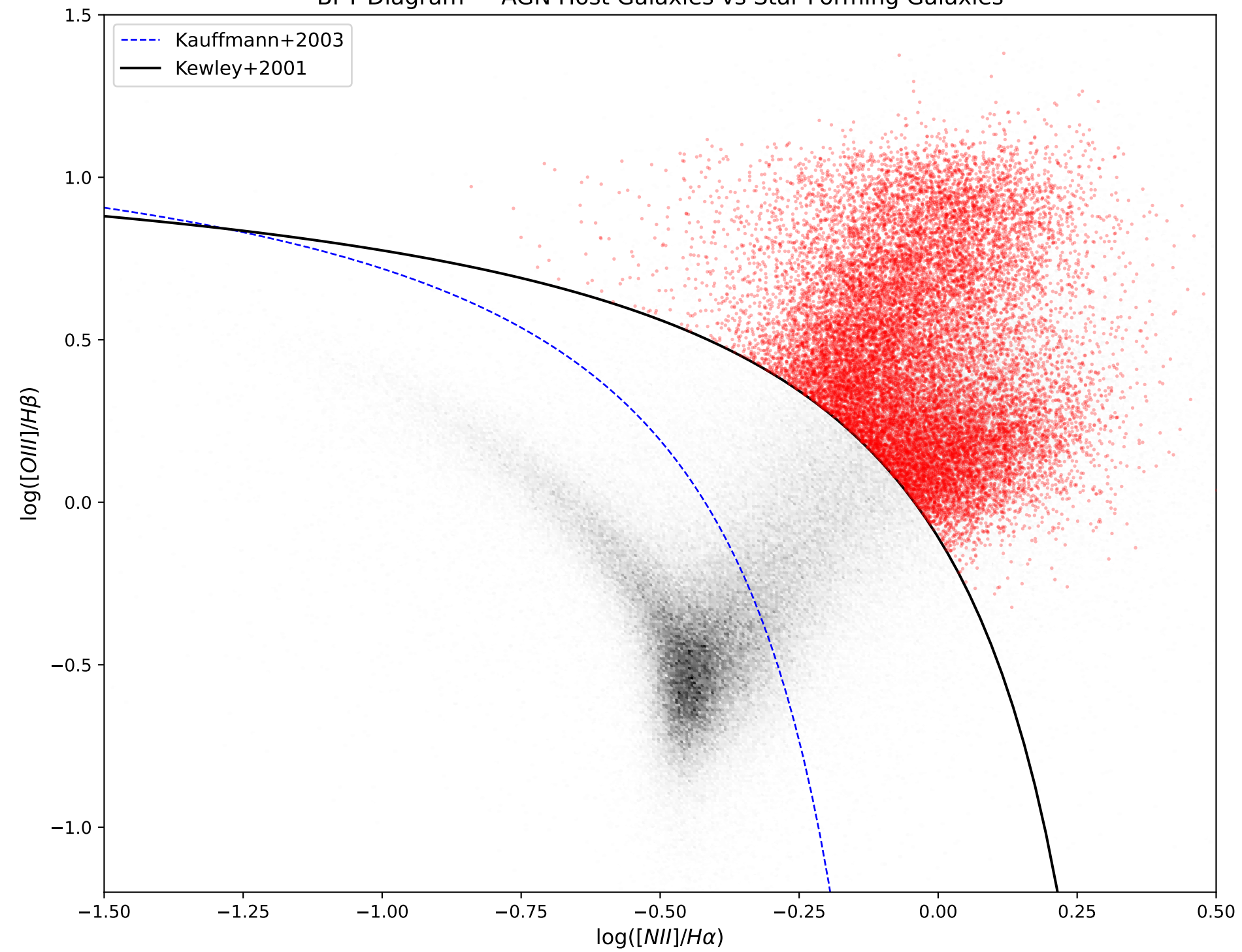
BPT Diagram — AGN Host Galaxies vs Star Forming Galaxies
